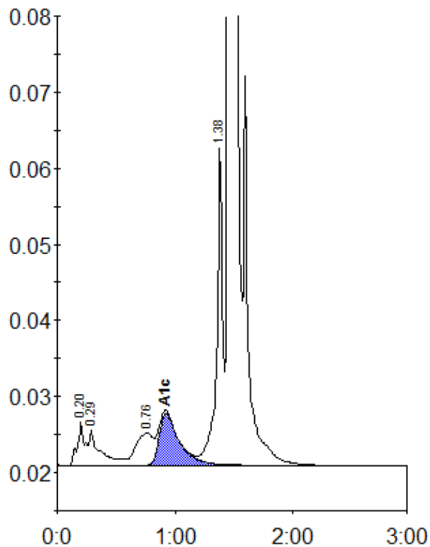
Peak table - ID: 10404366
